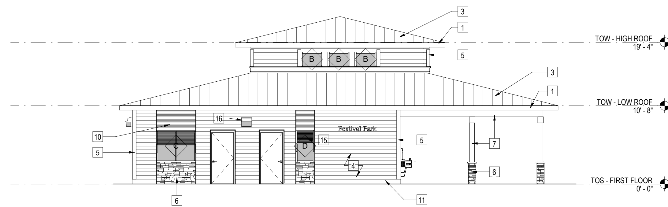
④ SOUTH ELEVATION 1/8" = 1'-0"
