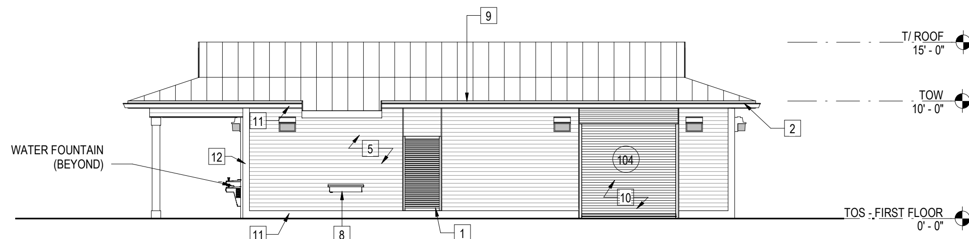
③ EAST ELEVATION 1/8" = 1'-0"
