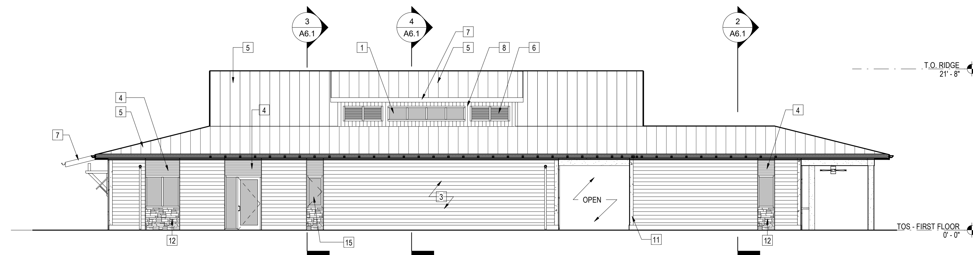
④ EAST ELEVATION 1/8" = 1'-0"
