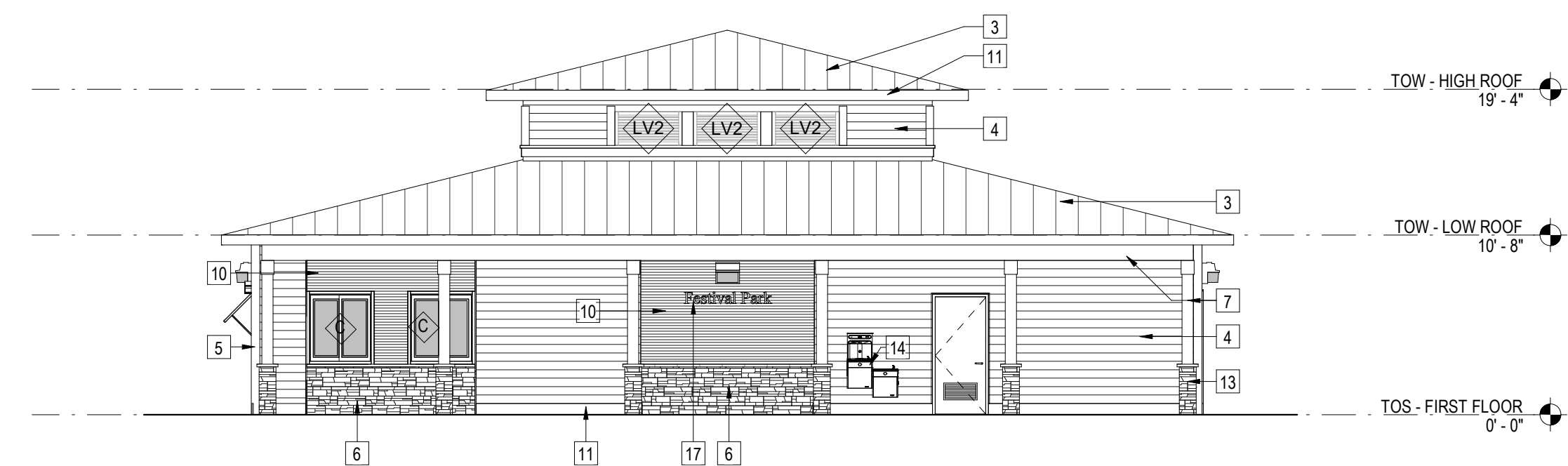
① EAST ELEVATION 1/8" = 1'-0"
