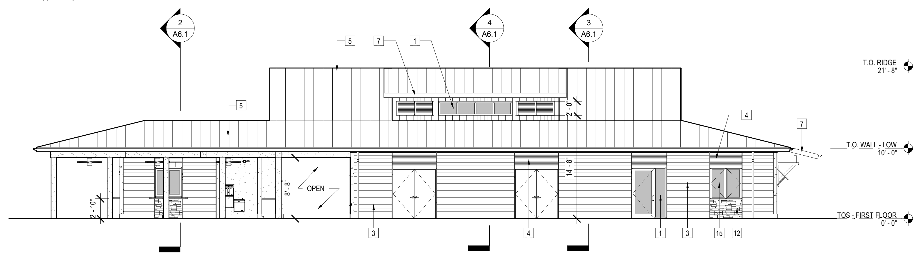
② WEST ELEVATION 1/8" = 1'-0"
