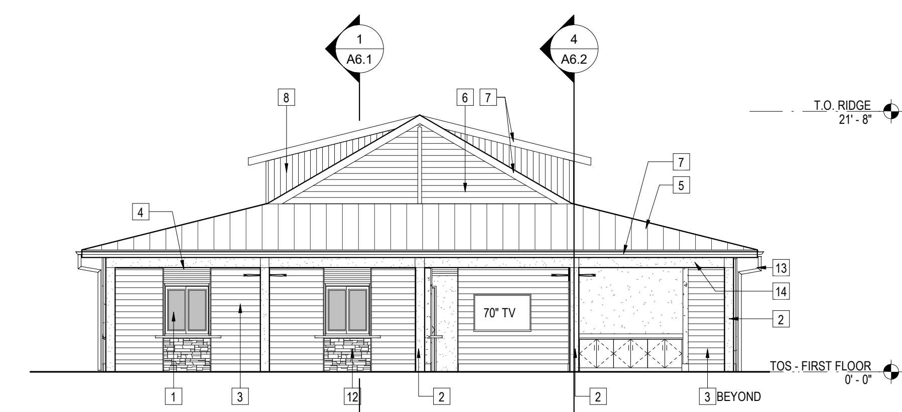
③ NORTH ELEVATION 1/8" = 1'-0"
