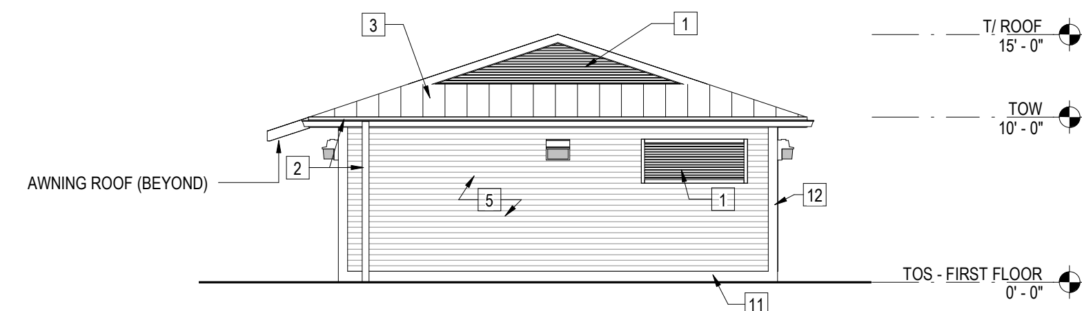
④ NORTH ELEVATION 1/8" = 1'-0"
