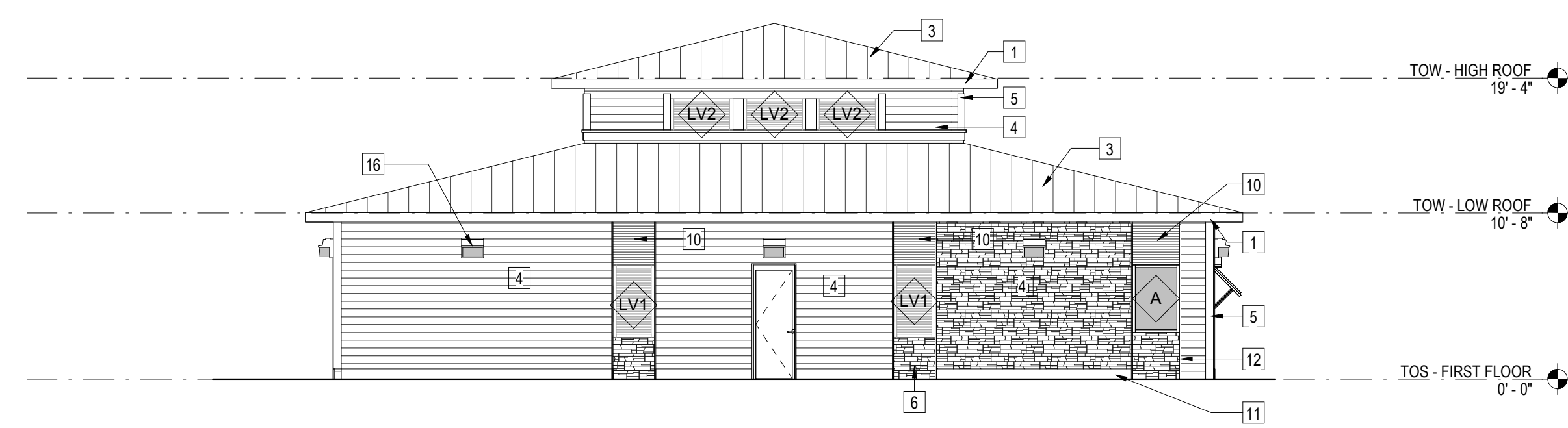
② WEST ELEVATION 1/8" = 1'-0"
