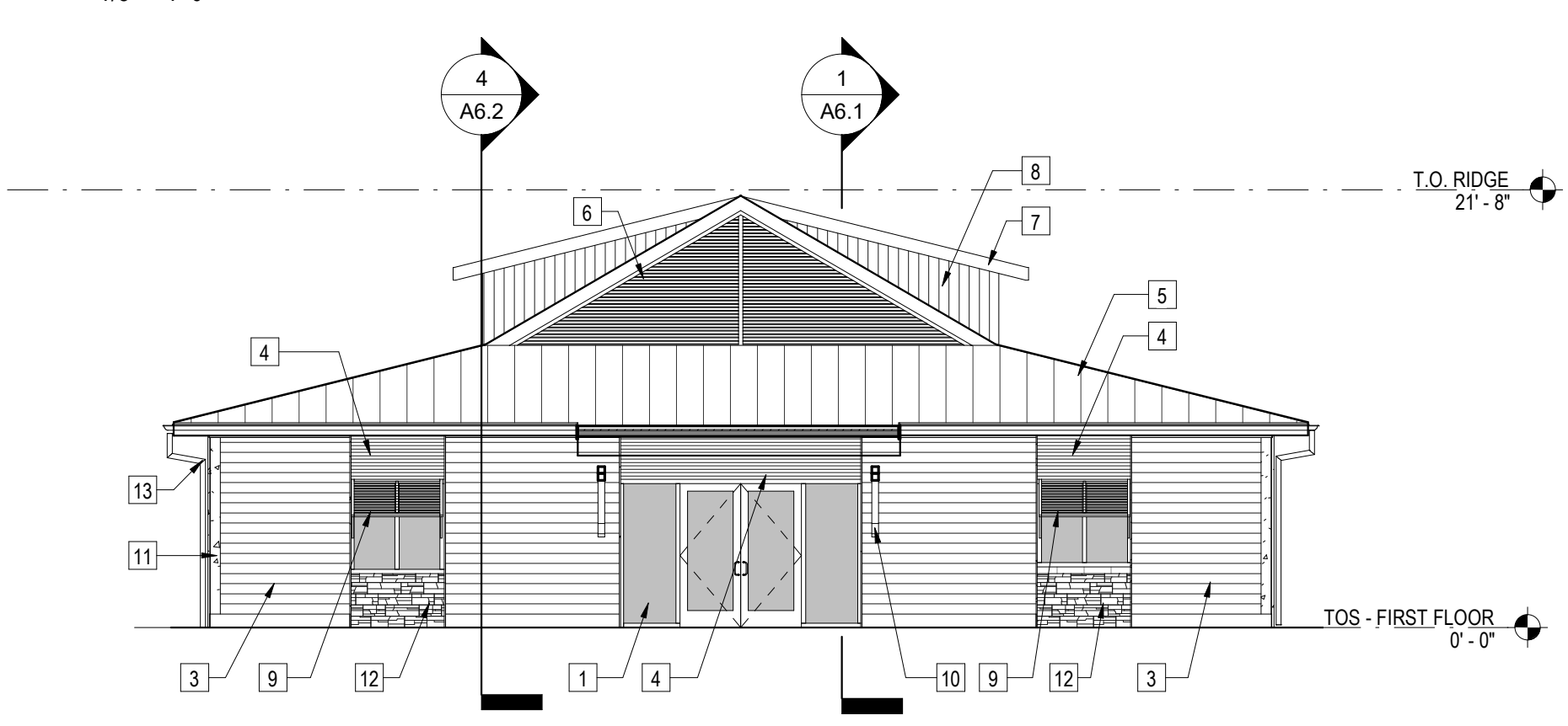
① SOUTH ELEVATION 1/8" = 1'-0"
